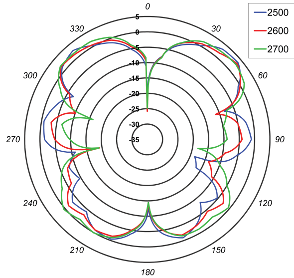
Vertical Plane (2500-2700 MHz)
