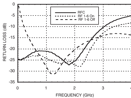
Return Loss [1]
